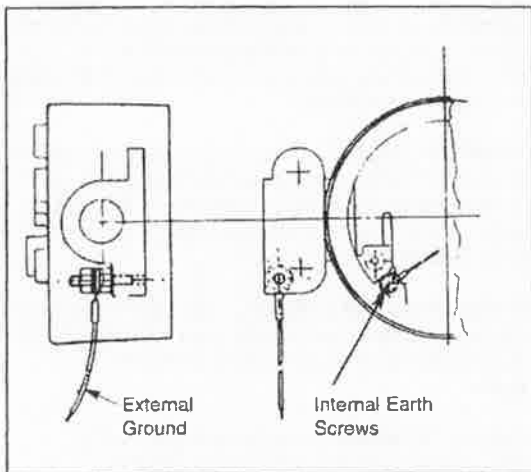
Figure 4. External/Internal Ground Connections
